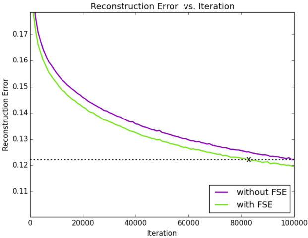
Fig. 8. The reconstruction error of architecture (c) with 3 frames during the training with and without Filter Symmetry Enforcement (FSE).
