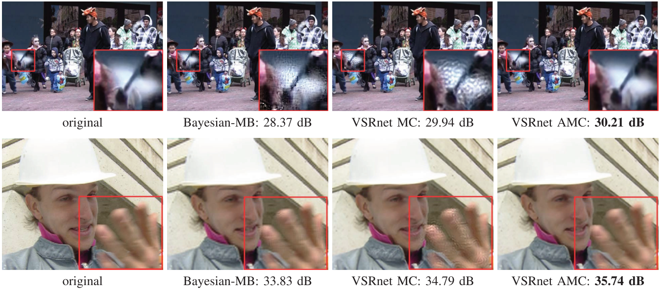
Fig. 10. Frames with motion blurred objects from the walk and foreman sequence, reconstructed with MC and AMC for upscale factor 3.
