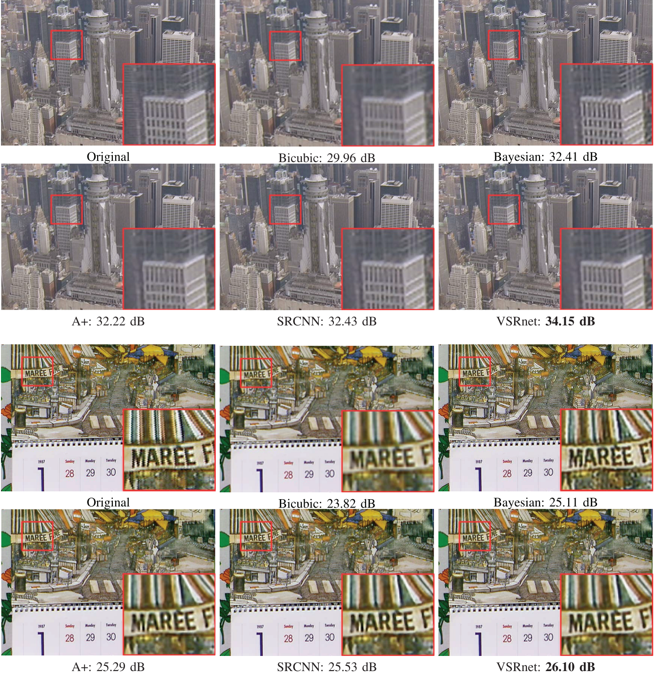
Fig. 5. Comparison to the State-of-the-Art: SR frames from the city and calendar videos compared to our method (VSRnet) for upscale factor 2.
